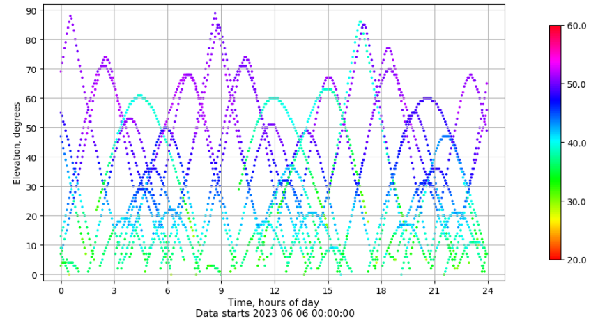
Time-elevation plot for station VIGO. Signal to Noise S1C Data file VIGO00ESP_R_2023157.xtr
