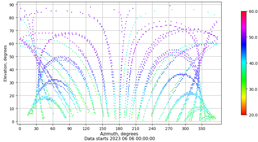
Azimuth-elevation plot for station VIGO. Signal to Noise S1C Data file VIGO00ESP_R_2023157.xtr
