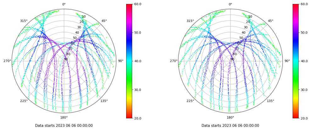
Skyplot for station VIGO. Signal to Noise S1C Data file VIGO00ESP_R_2023157.xtr Skyplot for station VIGO. Signal to Noise S2C Data file VIGO00ESP_R_2023157.xtr
