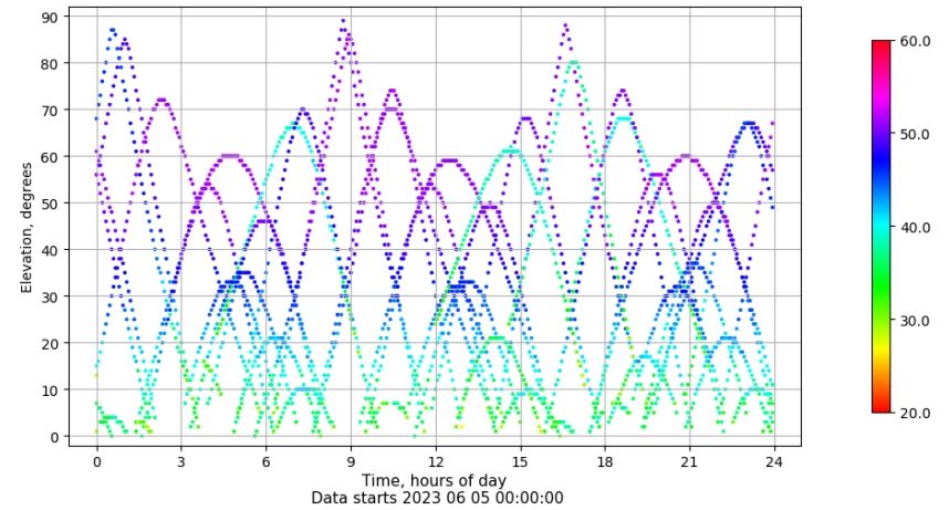
Time-elevation plot for station VIGO. Signal to Noise S1C Data file VIGO00ESP_R_2023156.xtr
