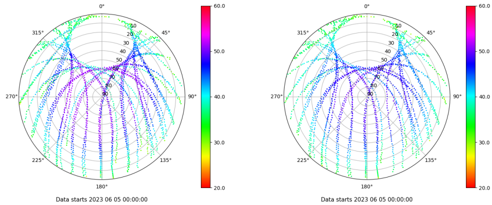
Skyplot for station VIGO. Signal to Noise S1C Data file VIGO00ESP_R_2023156.xtr Skyplot for station VIGO. Signal to Noise S2C Data file VIGO00ESP_R_2023156.xtr
