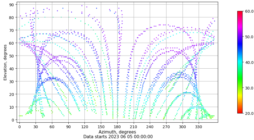
Azimuth-elevation plot for station VIGO. Signal to Noise S1C Data file VIGO00ESP_R_2023156.xtr
