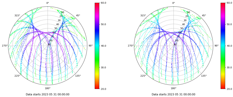
Skyplot for station VIGO. Signal to Noise S1C Data file VIGO00ESP_R_2023151.xtr Skyplot for station VIGO. Signal to Noise S2C Data file VIGO00ESP_R_2023151.xtr
