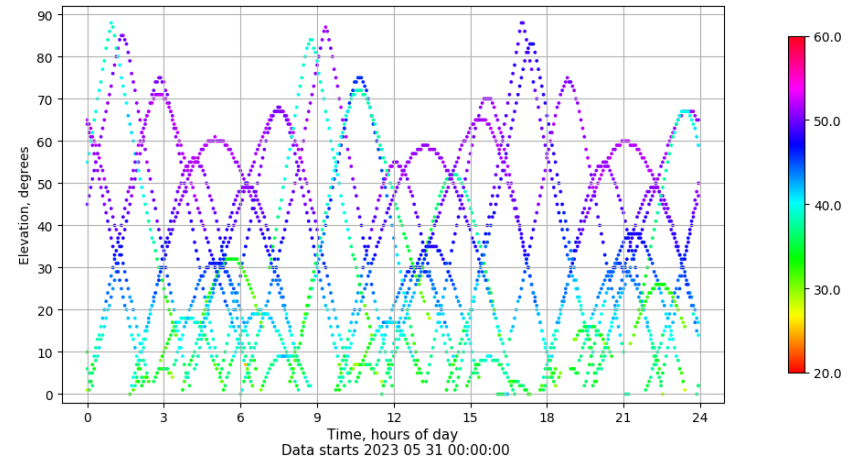
Time-elevation plot for station VIGO. Signal to Noise S1C Data file VIGO00ESP_R_2023151.xtr
