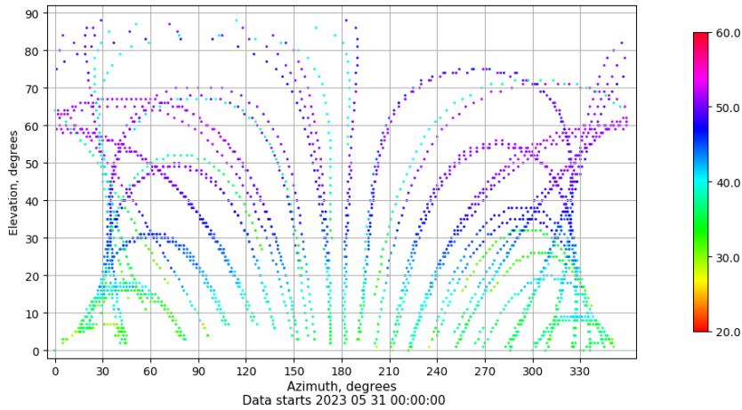
Azimuth-elevation plot for station VIGO. Signal to Noise S1C Data file VIGO00ESP_R_2023151.xtr
