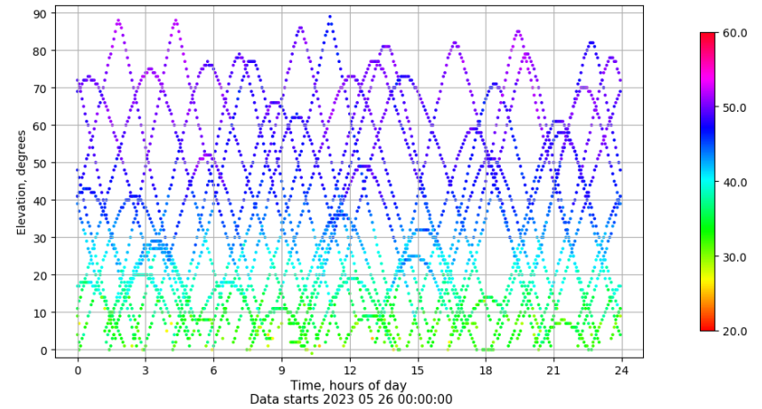
Time-elevation plot for station VIGO. Signal to Noise S1C Data file VIGO00ESP_R_2023146.xtr
