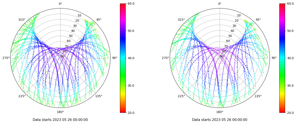
Skyplot for station VIGO. Signal to Noise S1C Data file VIGO00ESP_R_2023146.xtr Skyplot for station VIGO. Signal to Noise S2X Data file VIGO00ESP_R_2023146.xtr
