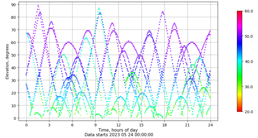
Time-elevation plot for station VIGO. Signal to Noise S1C Data file VIGO00ESP_R_2023144.xtr
