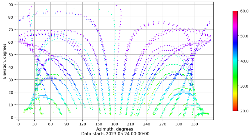
Azimuth-elevation plot for station VIGO. Signal to Noise S1C Data file VIGO00ESP_R_2023144.xtr
