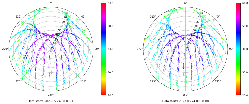
Skyplot for station VIGO. Signal to Noise S1C Data file VIGO00ESP_R_2023144.xtr Skyplot for station VIGO. Signal to Noise S2C Data file VIGO00ESP_R_2023144.xtr
