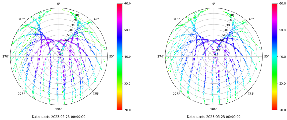
Skyplot for station VIGO. Signal to Noise S1C Data file VIGO00ESP_R_2023143.xtr Skyplot for station VIGO. Signal to Noise S2C Data file VIGO00ESP_R_2023143.xtr
