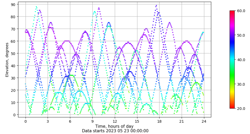
Time-elevation plot for station VIGO. Signal to Noise S1C Data file VIGO00ESP_R_2023143.xtr
