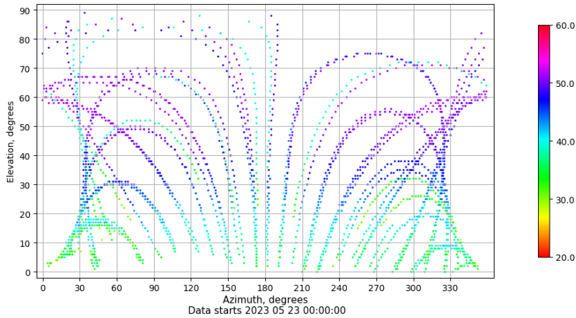
Azimuth-elevation plot for station VIGO. Signal to Noise S1C Data file VIGO00ESP_R_2023143.xtr
