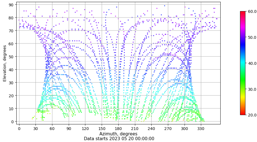
Azimuth-elevation plot for station VIGO. Signal to Noise S1C Data file VIGO00ESP_R_2023140.xtr
