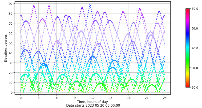
Time-elevation plot for station VIGO. Signal to Noise S1C Data file VIGO00ESP_R_2023140.xtr
