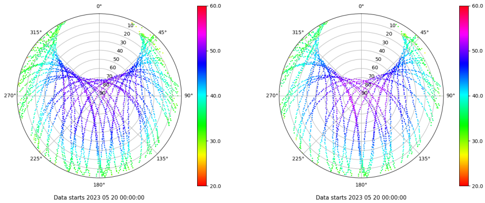
Skyplot for station VIGO. Signal to Noise S1C Data file VIGO00ESP_R_2023140.xtr Skyplot for station VIGO. Signal to Noise S2X Data file VIGO00ESP_R_2023140.xtr
