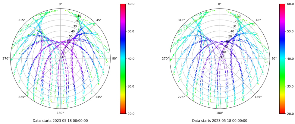
Skyplot for station VIGO. Signal to Noise S1C Data file VIGO00ESP_R_2023138.xtr Skyplot for station VIGO. Signal to Noise S2C Data file VIGO00ESP_R_2023138.xtr
