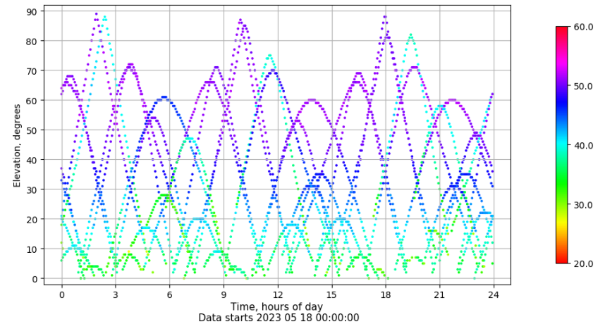
Time-elevation plot for station VIGO. Signal to Noise S1C Data file VIGO00ESP_R_2023138.xtr
