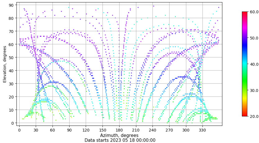
Azimuth-elevation plot for station VIGO. Signal to Noise S1C Data file VIGO00ESP_R_2023138.xtr
