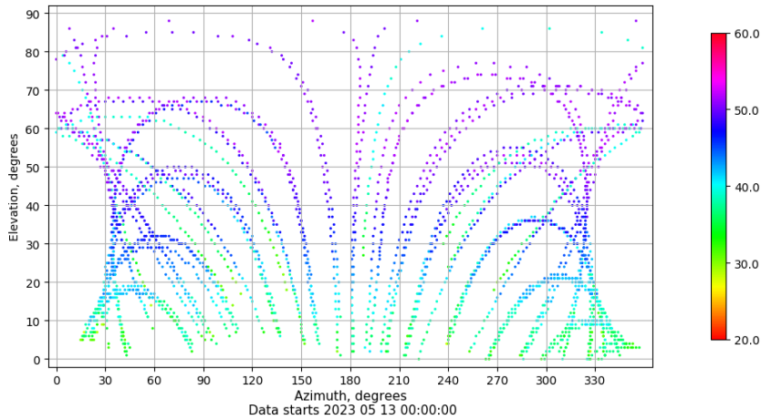
Azimuth-elevation plot for station VIGO. Signal to Noise S1C Data file VIGO00ESP_R_2023133.xtr
