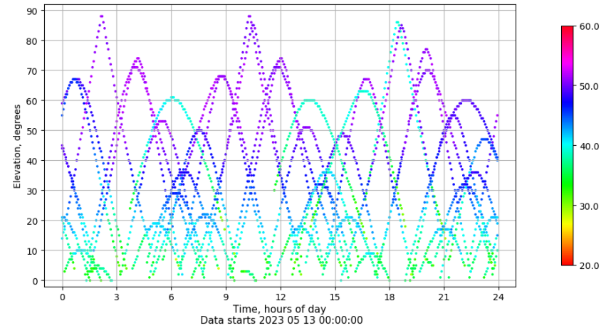
Time-elevation plot for station VIGO. Signal to Noise S1C Data file VIGO00ESP_R_2023133.xtr
