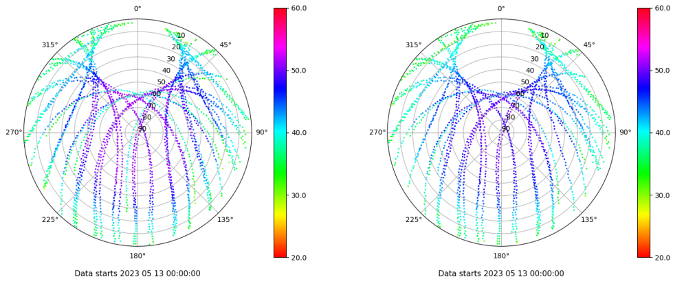
Skyplot for station VIGO. Signal to Noise S1C Data file VIGO00ESP_R_2023133.xtr Skyplot for station VIGO. Signal to Noise S2C Data file VIGO00ESP_R_2023133.xtr
