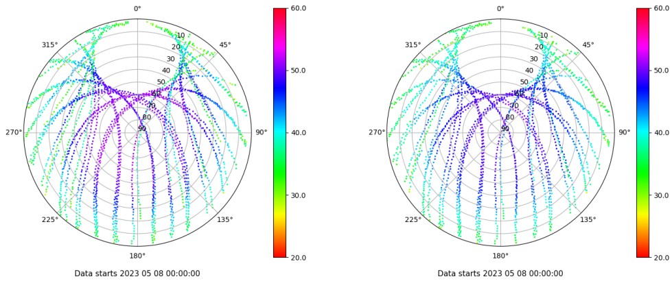
Skyplot for station VIGO. Signal to Noise S1C Data file VIGO00ESP_R_2023128.xtr Skyplot for station VIGO. Signal to Noise S2C Data file VIGO00ESP_R_2023128.xtr
