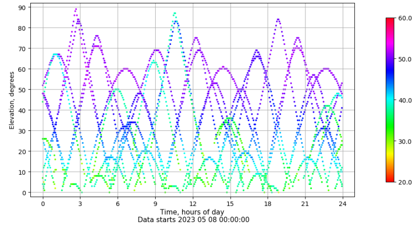
Time-elevation plot for station VIGO. Signal to Noise S1C Data file VIGO00ESP_R_2023128.xtr
