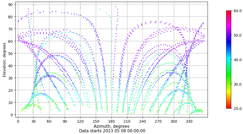
Azimuth-elevation plot for station VIGO. Signal to Noise S1C Data file VIGO00ESP_R_2023128.xtr
