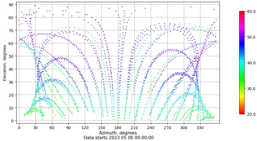
Azimuth-elevation plot for station VIGO. Signal to Noise S1C Data file VIGO00ESP_R_2023126.xtr
