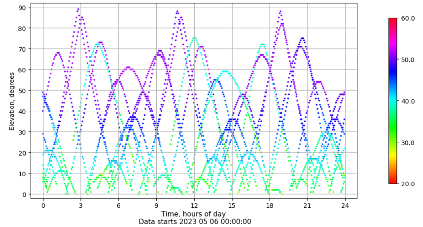
Time-elevation plot for station VIGO. Signal to Noise S1C Data file VIGO00ESP_R_2023126.xtr
