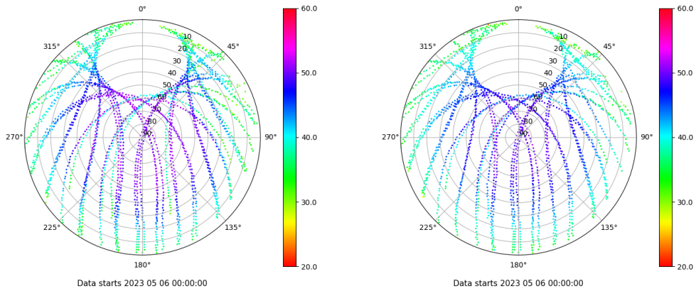
Skyplot for station VIGO. Signal to Noise S1C Data file VIGO00ESP_R_2023126.xtr Skyplot for station VIGO. Signal to Noise S2C Data file VIGO00ESP_R_2023126.xtr
