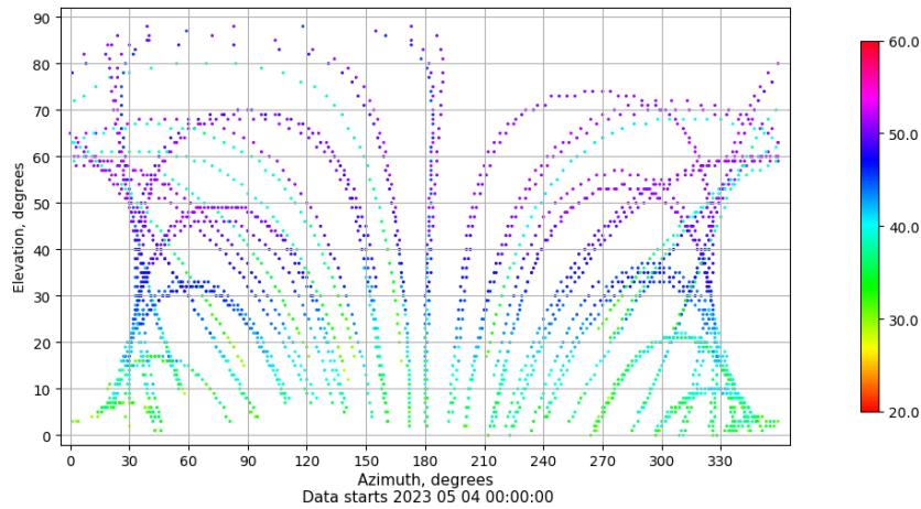
Azimuth-elevation plot for station VIGO. Signal to Noise S1C Data file VIGO00ESP_R_2023124.xtr
