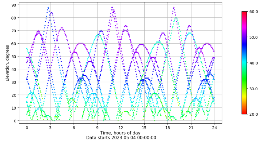
Time-elevation plot for station VIGO. Signal to Noise S1C Data file VIGO00ESP_R_2023124.xtr
