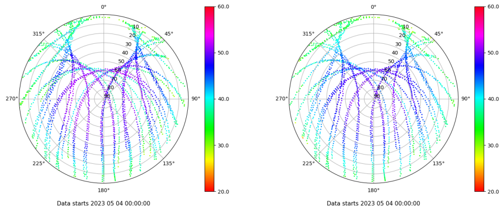
Skyplot for station VIGO. Signal to Noise S1C Data file VIGO00ESP_R_2023124.xtr Skyplot for station VIGO. Signal to Noise S2C Data file VIGO00ESP_R_2023124.xtr
