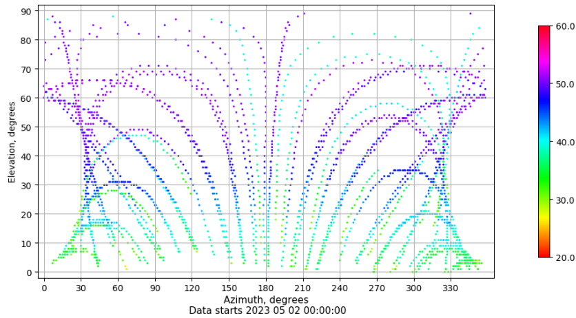
Azimuth-elevation plot for station VIGO. Signal to Noise S1C Data file VIGO00ESP_R_2023122.xtr
