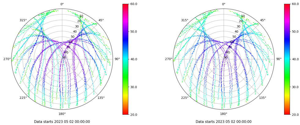
Skyplot for station VIGO. Signal to Noise S1C Data file VIGO00ESP_R_2023122.xtr Skyplot for station VIGO. Signal to Noise S2C Data file VIGO00ESP_R_2023122.xtr
