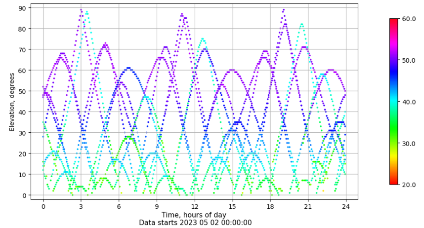
Time-elevation plot for station VIGO. Signal to Noise S1C Data file VIGO00ESP_R_2023122.xtr
