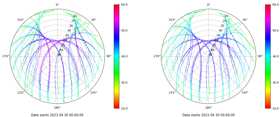
Skyplot for station VIGO. Signal to Noise S1C Data file VIGO00ESP_R_2023120.xtr Skyplot for station VIGO. Signal to Noise S2C Data file VIGO00ESP_R_2023120.xtr
