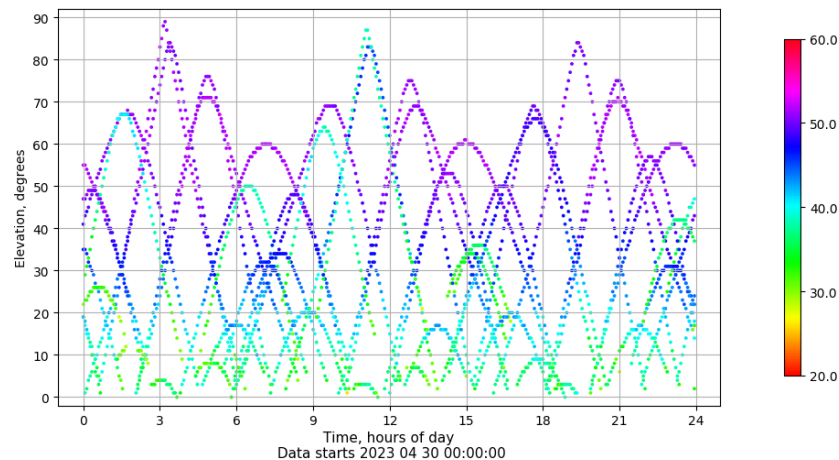
Time-elevation plot for station VIGO. Signal to Noise S1C Data file VIGO00ESP_R_2023120.xtr
