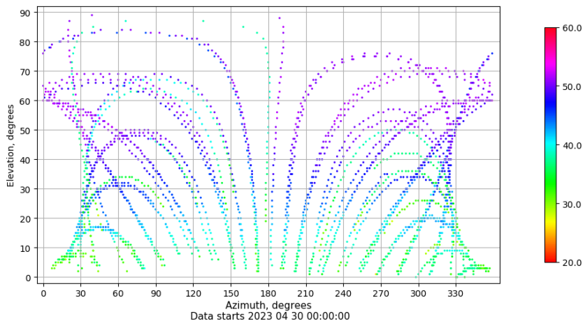
Azimuth-elevation plot for station VIGO. Signal to Noise S1C Data file VIGO00ESP_R_2023120.xtr
