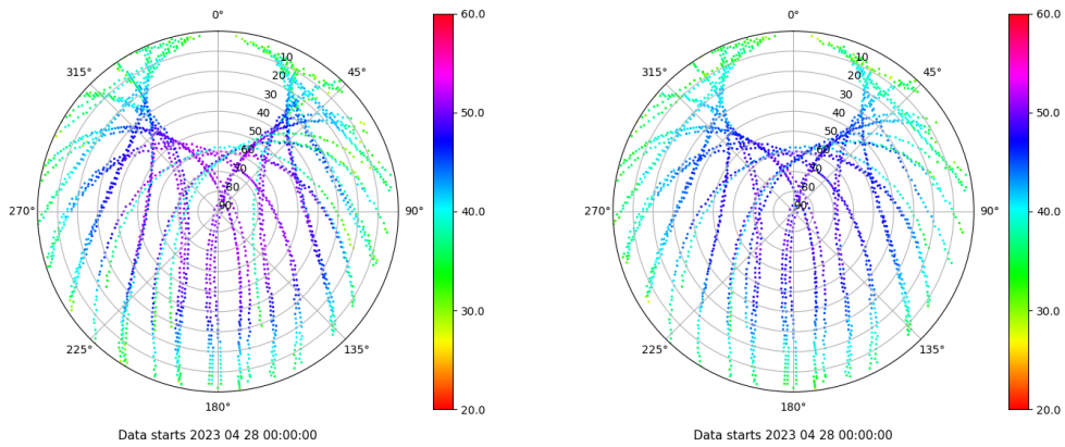
Skyplot for station VIGO. Signal to Noise S1C Data file VIGO00ESP_R_2023118.xtr Skyplot for station VIGO. Signal to Noise S2C Data file VIGO00ESP_R_2023118.xtr
