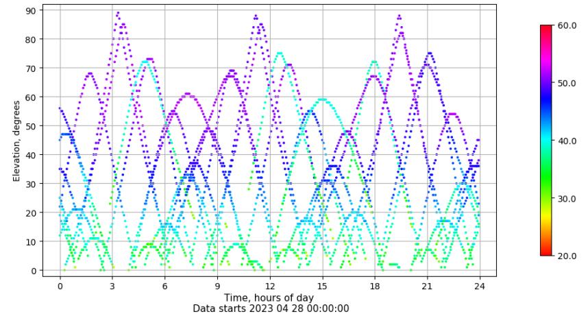
Time-elevation plot for station VIGO. Signal to Noise S1C Data file VIGO00ESP_R_2023118.xtr
