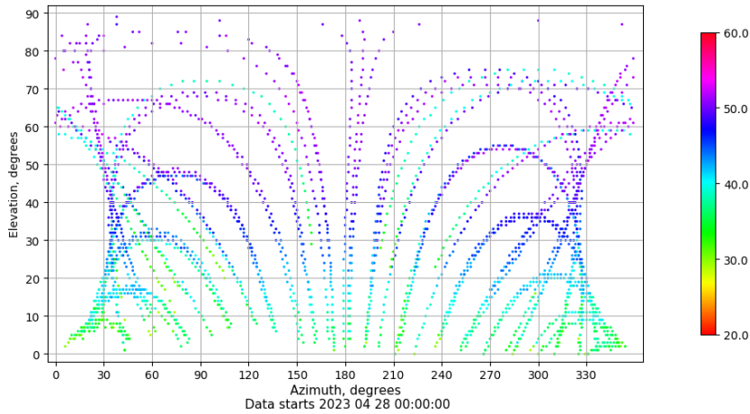
Azimuth-elevation plot for station VIGO. Signal to Noise S1C Data file VIGO00ESP_R_2023118.xtr
