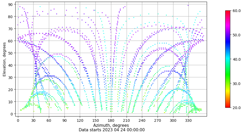
Azimuth-elevation plot for station VIGO. Signal to Noise S1C Data file VIGO00ESP_R_2023114.xtr
