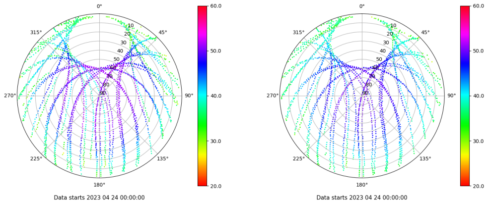
Skyplot for station VIGO. Signal to Noise S1C Data file VIGO00ESP_R_2023114.xtr Skyplot for station VIGO. Signal to Noise S2C Data file VIGO00ESP_R_2023114.xtr
