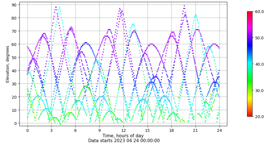
Time-elevation plot for station VIGO. Signal to Noise S1C Data file VIGO00ESP_R_2023114.xtr
