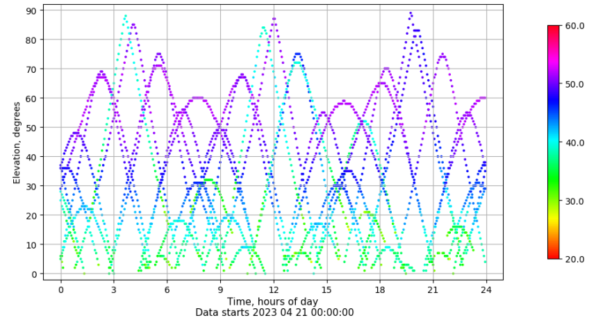
Time-elevation plot for station VIGO. Signal to Noise S1C Data file VIGO00ESP_R_2023111.xtr
