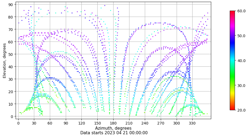
Azimuth-elevation plot for station VIGO. Signal to Noise S1C Data file VIGO00ESP_R_2023111.xtr
