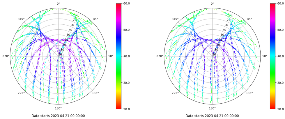
Skyplot for station VIGO. Signal to Noise S1C Data file VIGO00ESP_R_2023111.xtr Skyplot for station VIGO. Signal to Noise S2C Data file VIGO00ESP_R_2023111.xtr
