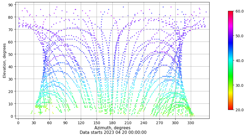
Azimuth-elevation plot for station VIGO. Signal to Noise S1C Data file VIGO00ESP_R_2023110.xtr
