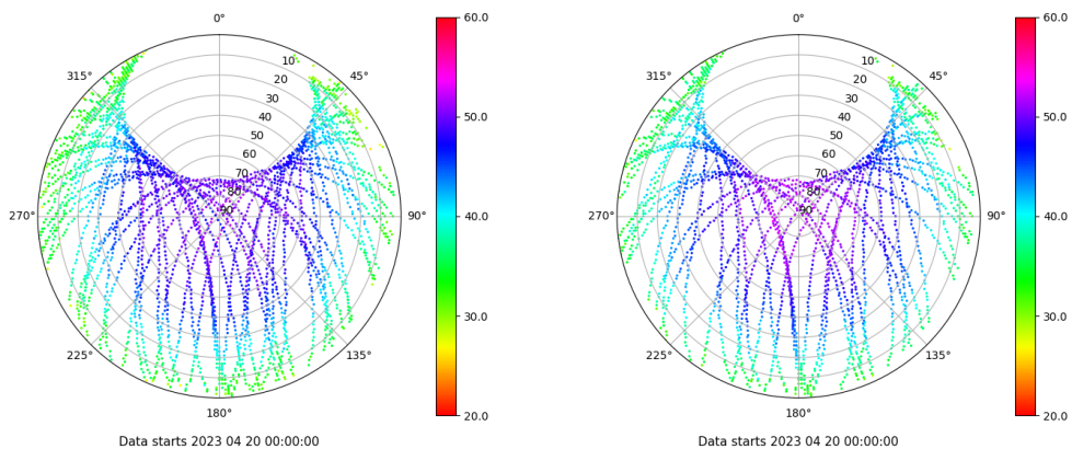
Skyplot for station VIGO. Signal to Noise S1C Data file VIGO00ESP_R_2023110.xtr Skyplot for station VIGO. Signal to Noise S2X Data file VIGO00ESP_R_2023110.xtr
