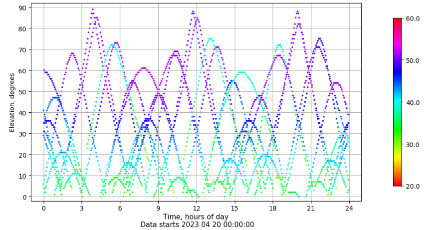
Time-elevation plot for station VIGO. Signal to Noise S1C Data file VIGO00ESP_R_2023110.xtr
