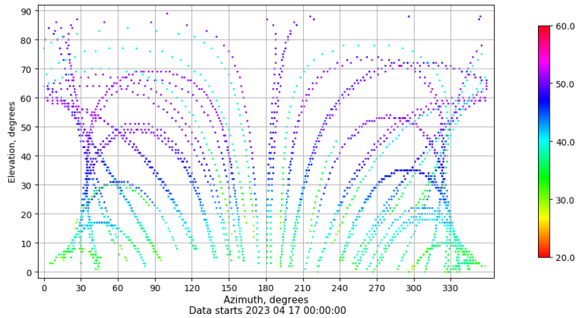
Azimuth-elevation plot for station VIGO. Signal to Noise S1C Data file VIGO00ESP_R_2023107.xtr
