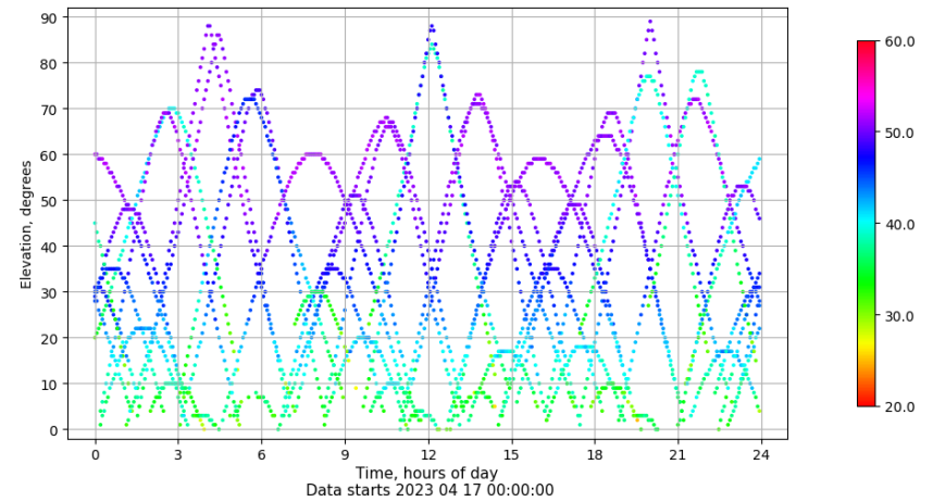
Time-elevation plot for station VIGO. Signal to Noise S1C Data file VIGO00ESP_R_2023107.xtr
