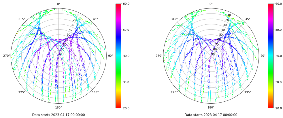
Skyplot for station VIGO. Signal to Noise S1C Data file VIGO00ESP_R_2023107.xtr Skyplot for station VIGO. Signal to Noise S2C Data file VIGO00ESP_R_2023107.xtr
