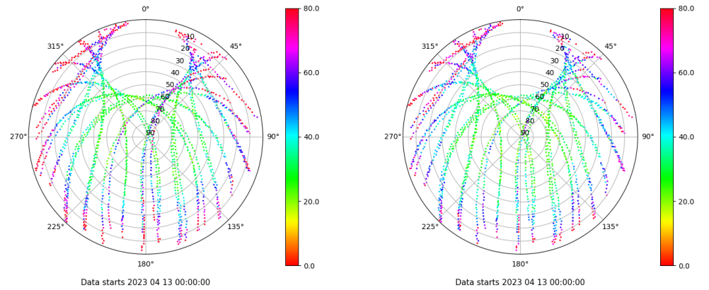
Skyplot for station VIGO. Parameter M1C Data file VIGO00ESP_R_2023103.xtr Skyplot for station VIGO. Parameter M2C Data file VIGO00ESP_R_2023103.xtr
