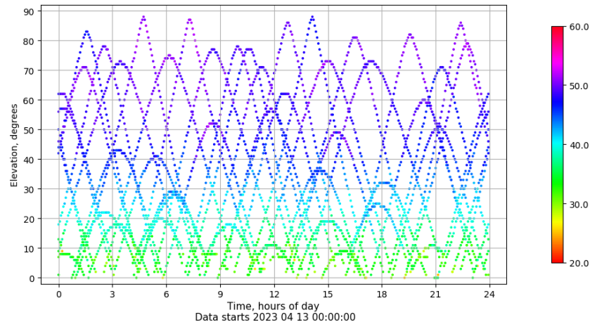
Time-elevation plot for station VIGO. Signal to Noise S1C Data file VIGO00ESP_R_2023103.xtr
