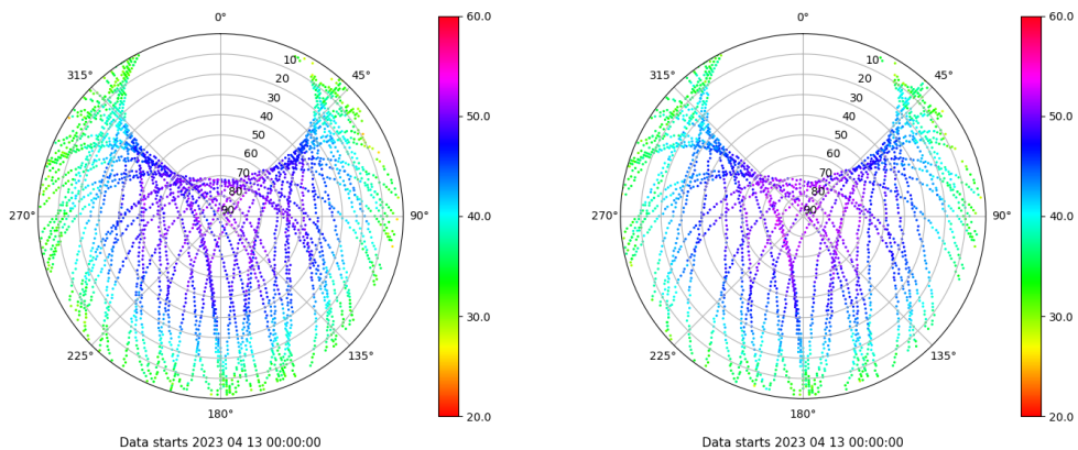
Skyplot for station VIGO. Signal to Noise S1C Data file VIGO00ESP_R_2023103.xtr Skyplot for station VIGO. Signal to Noise S2X Data file VIGO00ESP_R_2023103.xtr
