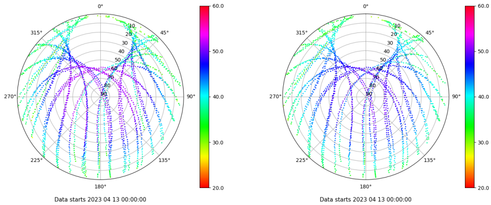
Skyplot for station VIGO. Signal to Noise S1C Data file VIGO00ESP_R_2023103.xtr Skyplot for station VIGO. Signal to Noise S2C Data file VIGO00ESP_R_2023103.xtr
