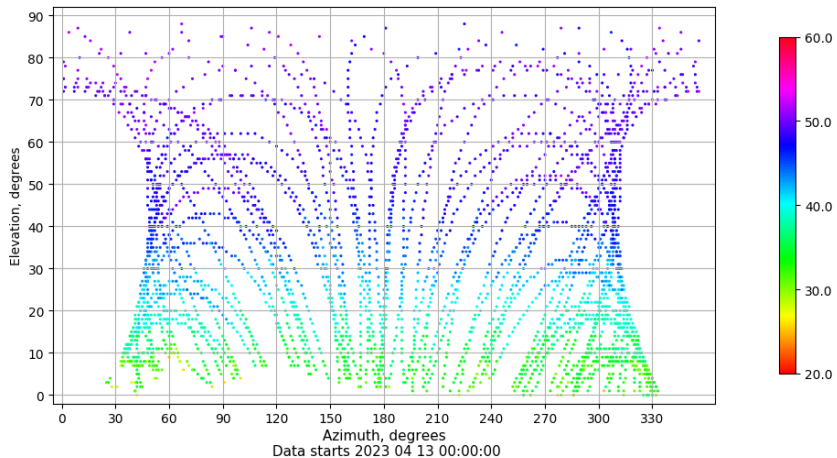
Azimuth-elevation plot for station VIGO. Signal to Noise S1C Data file VIGO00ESP_R_2023103.xtr
