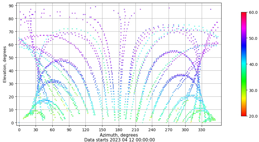
Azimuth-elevation plot for station VIGO. Signal to Noise S1C Data file VIGO00ESP_R_2023102.xtr
