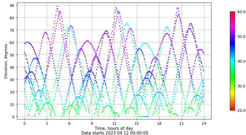
Time-elevation plot for station VIGO. Signal to Noise S1C Data file VIGO00ESP_R_2023102.xtr
