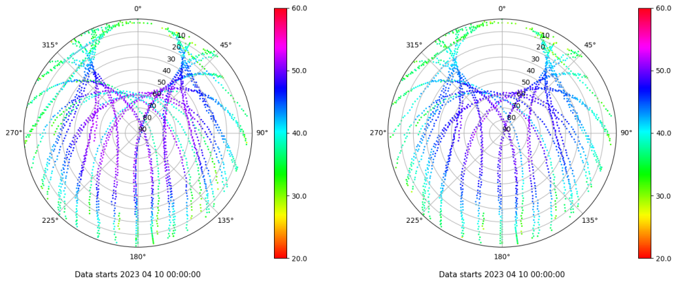
Skyplot for station VIGO. Signal to Noise S1C Data file VIGO00ESP_R_2023100.xtr Skyplot for station VIGO. Signal to Noise S2C Data file VIGO00ESP_R_2023100.xtr
