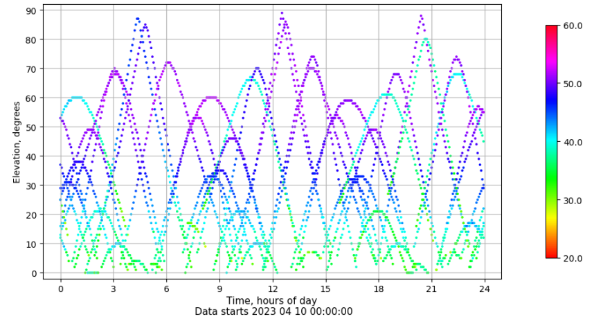
Time-elevation plot for station VIGO. Signal to Noise S1C Data file VIGO00ESP_R_2023100.xtr
