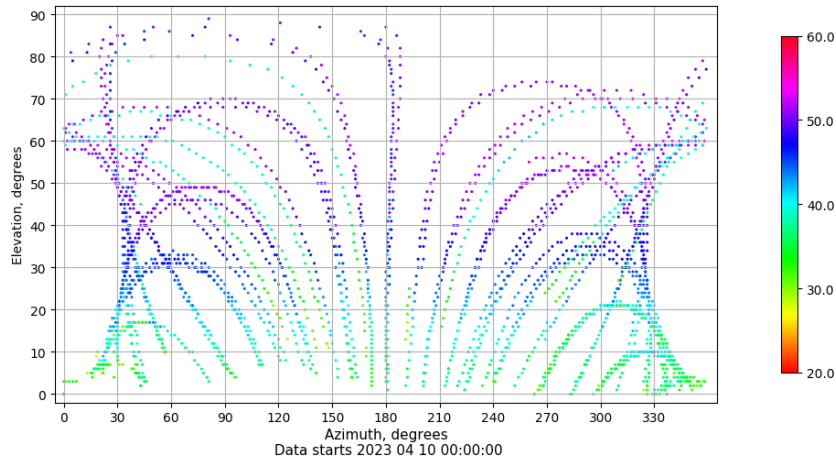
Azimuth-elevation plot for station VIGO. Signal to Noise S1C Data file VIGO00ESP_R_2023100.xtr
