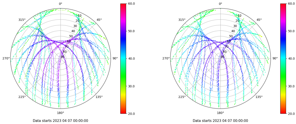
Skyplot for station VIGO. Signal to Noise S1C Data file VIGO00ESP_R_2023097.xtr Skyplot for station VIGO. Signal to Noise S2C Data file VIGO00ESP_R_2023097.xtr
