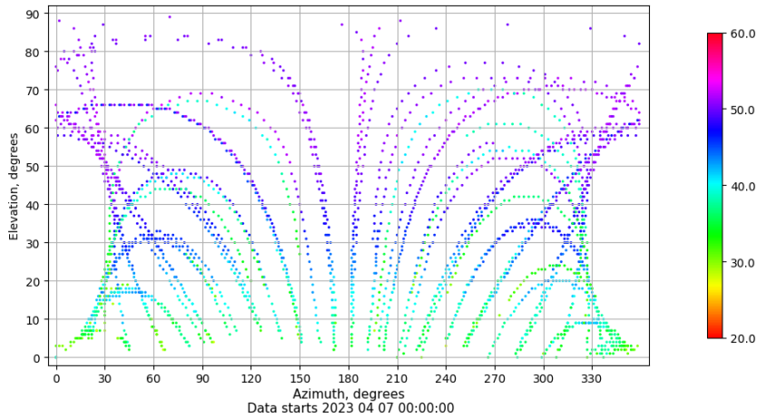
Azimuth-elevation plot for station VIGO. Signal to Noise S1C Data file VIGO00ESP_R_2023097.xtr
