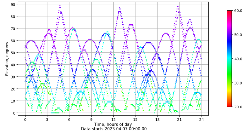
Time-elevation plot for station VIGO. Signal to Noise S1C Data file VIGO00ESP_R_2023097.xtr
