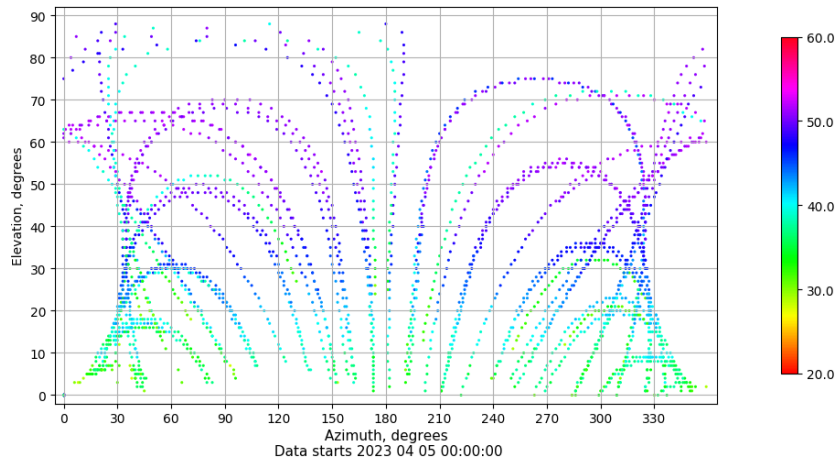
Azimuth-elevation plot for station VIGO. Signal to Noise S1C Data file VIGO00ESP_R_2023095.xtr
