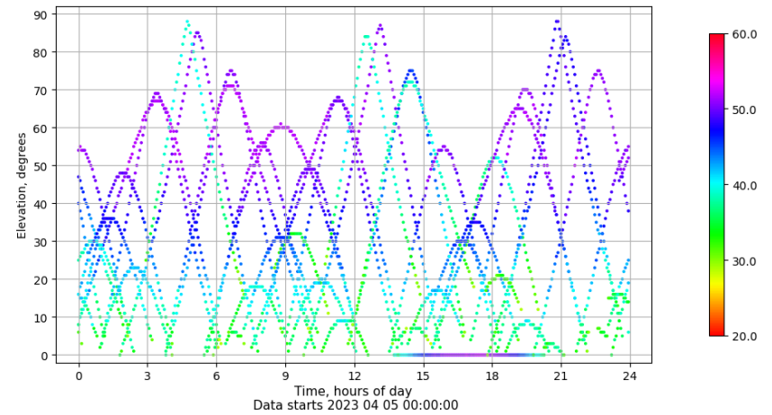
Time-elevation plot for station VIGO. Signal to Noise S1C Data file VIGO00ESP_R_2023095.xtr
