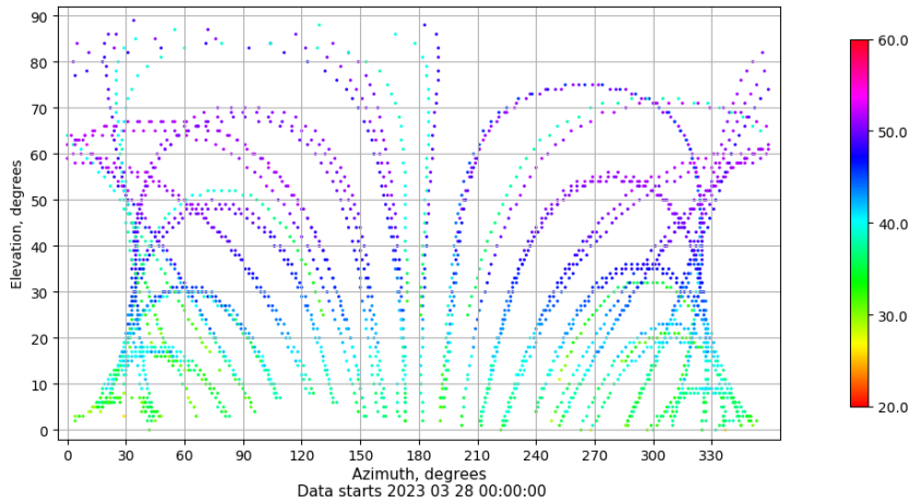
Azimuth-elevation plot for station VIGO. Signal to Noise S1C Data file VIGO00ESP_R_2023087.xtr
