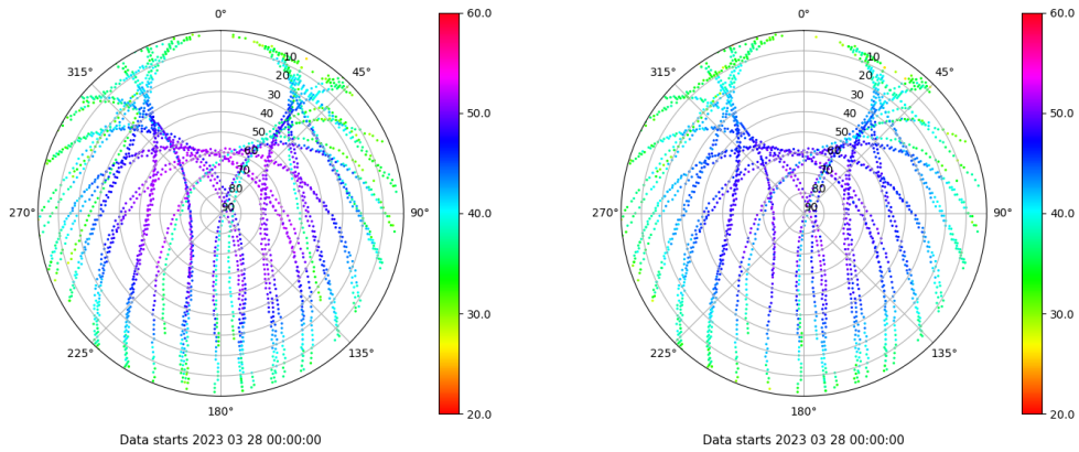
Skyplot for station VIGO. Signal to Noise S1C Data file VIGO00ESP_R_2023087.xtr Skyplot for station VIGO. Signal to Noise S2C Data file VIGO00ESP_R_2023087.xtr
