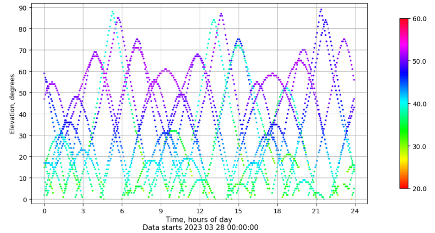
Time-elevation plot for station VIGO. Signal to Noise S1C Data file VIGO00ESP_R_2023087.xtr
