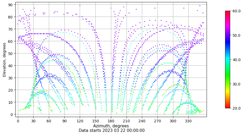
Azimuth-elevation plot for station VIGO. Signal to Noise S1C Data file VIGO00ESP_R_2023081.xtr
