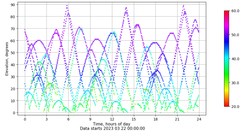
Time-elevation plot for station VIGO. Signal to Noise S1C Data file VIGO00ESP_R_2023081.xtr
