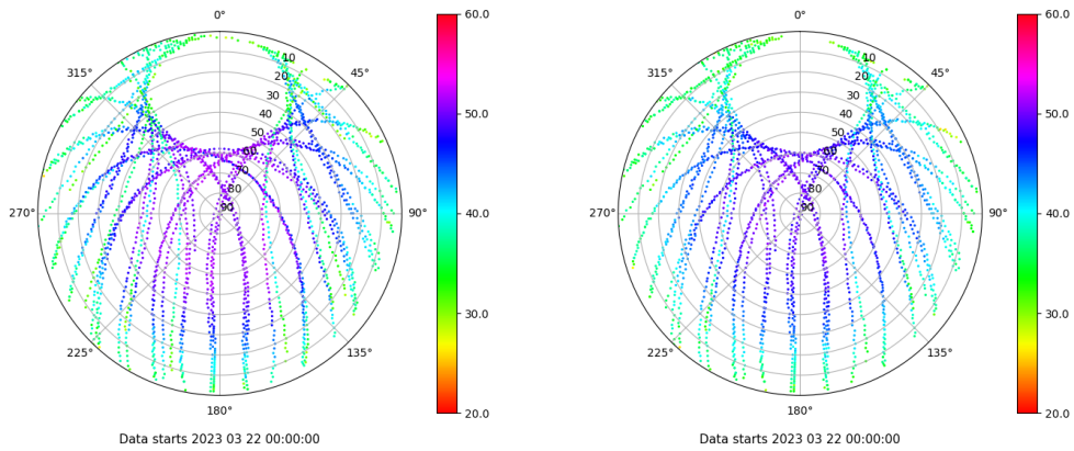
Skyplot for station VIGO. Signal to Noise S1C Data file VIGO00ESP_R_2023081.xtr Skyplot for station VIGO. Signal to Noise S2C Data file VIGO00ESP_R_2023081.xtr
