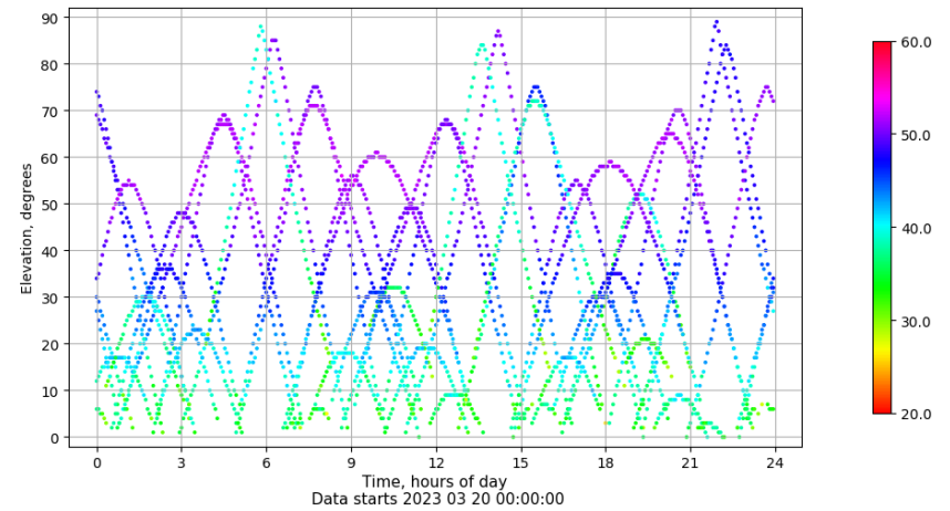
Time-elevation plot for station VIGO. Signal to Noise S1C Data file VIGO00ESP_R_2023079.xtr
