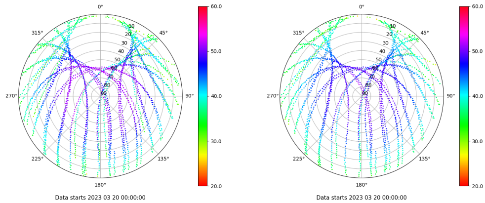
Skyplot for station VIGO. Signal to Noise S1C Data file VIGO00ESP_R_2023079.xtr Skyplot for station VIGO. Signal to Noise S2C Data file VIGO00ESP_R_2023079.xtr
