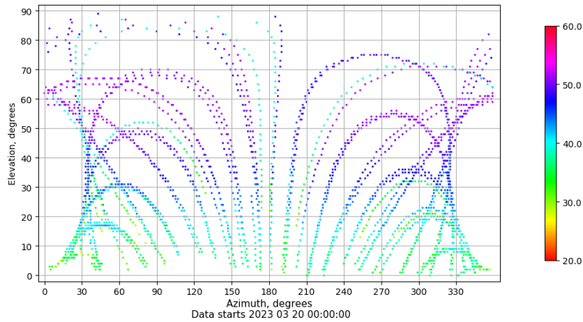
Azimuth-elevation plot for station VIGO. Signal to Noise S1C Data file VIGO00ESP_R_2023079.xtr
