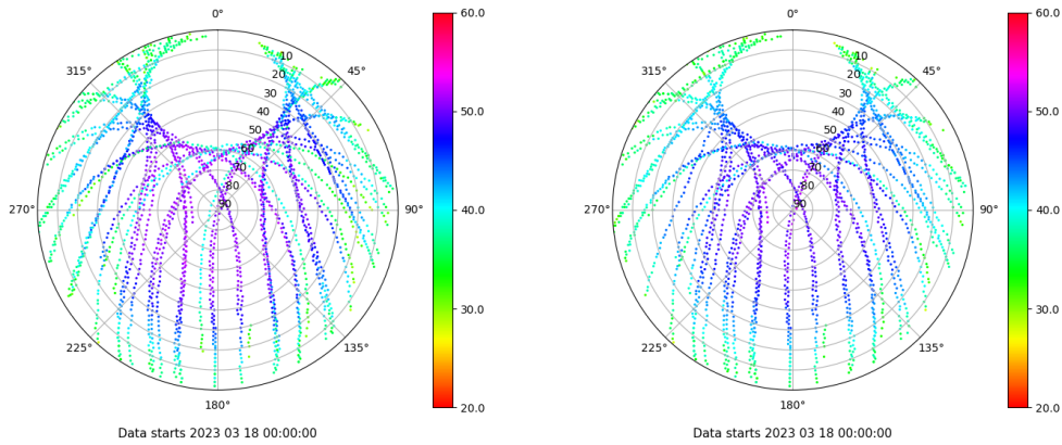
Skyplot for station VIGO. Signal to Noise S1C Data file VIGO00ESP_R_2023077.xtr Skyplot for station VIGO. Signal to Noise S2C Data file VIGO00ESP_R_2023077.xtr
