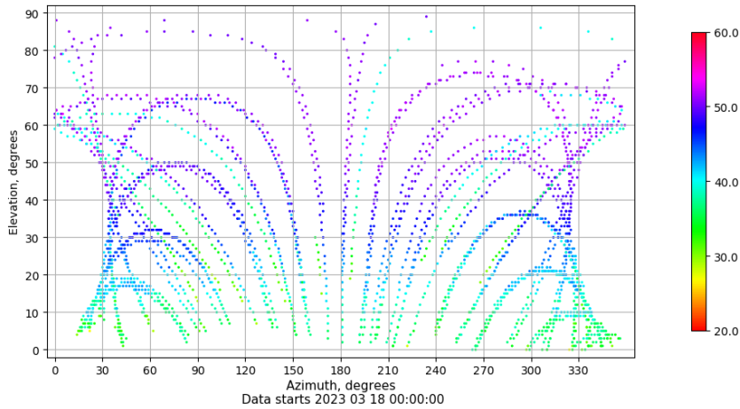
Azimuth-elevation plot for station VIGO. Signal to Noise S1C Data file VIGO00ESP_R_2023077.xtr
