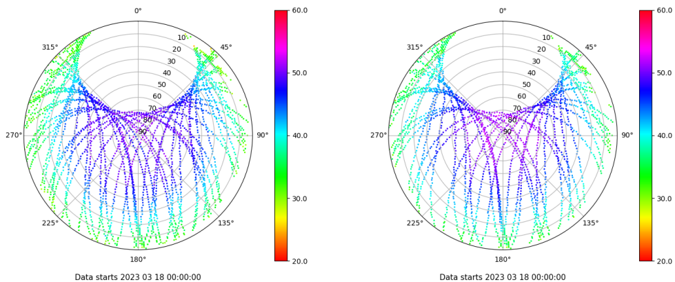
Skyplot for station VIGO. Signal to Noise S1C Data file VIGO00ESP_R_2023077.xtr Skyplot for station VIGO. Signal to Noise S2X Data file VIGO00ESP_R_2023077.xtr
