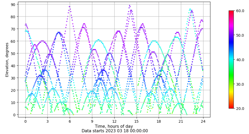
Time-elevation plot for station VIGO. Signal to Noise S1C Data file VIGO00ESP_R_2023077.xtr
