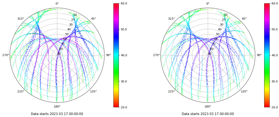
Skyplot for station VIGO. Signal to Noise S1C Data file VIGO00ESP_R_2023076.xtr Skyplot for station VIGO. Signal to Noise S2C Data file VIGO00ESP_R_2023076.xtr
