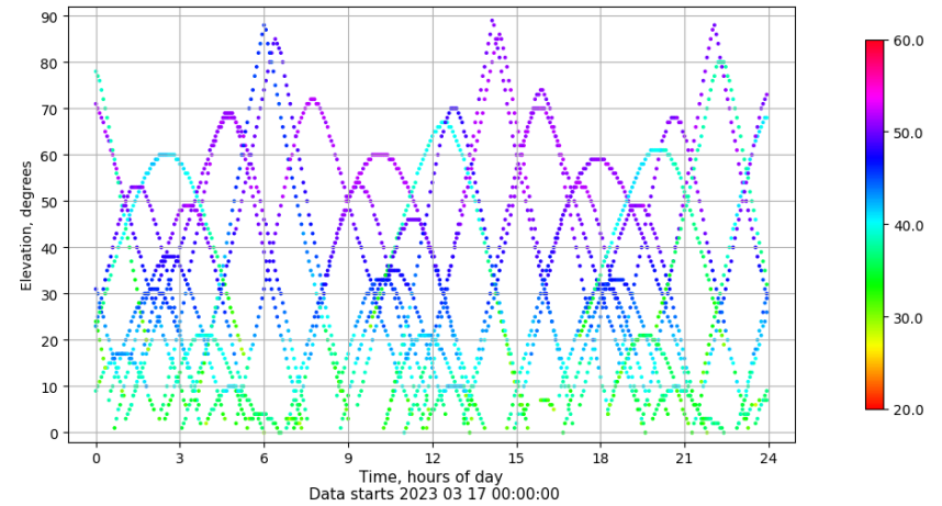
Time-elevation plot for station VIGO. Signal to Noise S1C Data file VIGO00ESP_R_2023076.xtr
