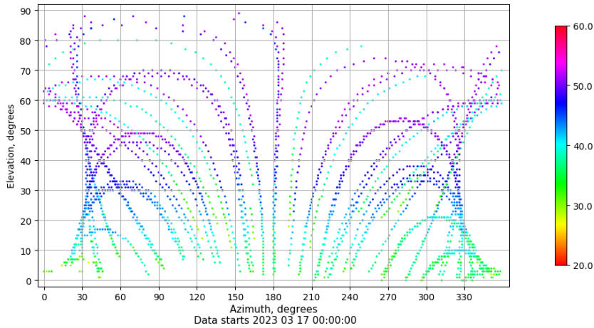
Azimuth-elevation plot for station VIGO. Signal to Noise S1C Data file VIGO00ESP_R_2023076.xtr
