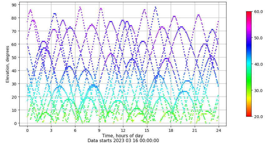
Time-elevation plot for station VIGO. Signal to Noise S1C Data file VIGO00ESP_R_2023075.xtr
