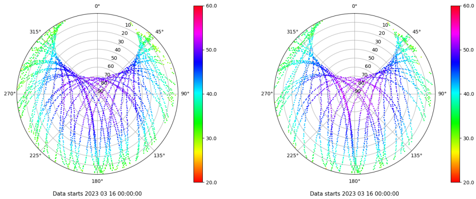
Skyplot for station VIGO. Signal to Noise S1C Data file VIGO00ESP_R_2023075.xtr Skyplot for station VIGO. Signal to Noise S2X Data file VIGO00ESP_R_2023075.xtr
