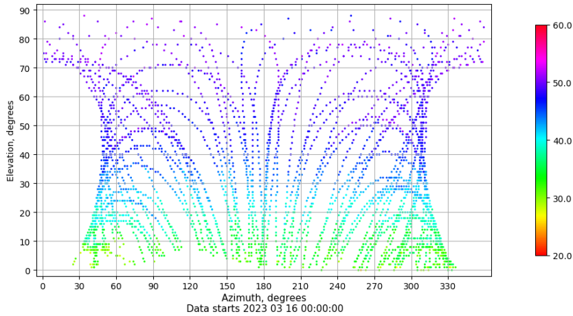
Azimuth-elevation plot for station VIGO. Signal to Noise S1C Data file VIGO00ESP_R_2023075.xtr
