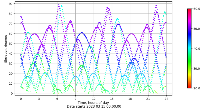
Time-elevation plot for station VIGO. Signal to Noise S1C Data file VIGO00ESP_R_2023074.xtr
