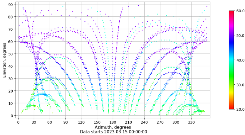
Azimuth-elevation plot for station VIGO. Signal to Noise S1C Data file VIGO00ESP_R_2023074.xtr
