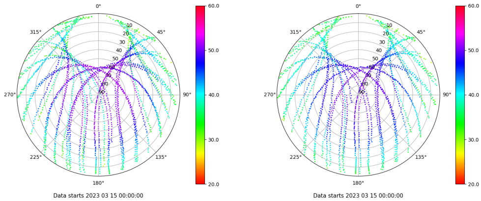
Skyplot for station VIGO. Signal to Noise S1C Data file VIGO00ESP_R_2023074.xtr Skyplot for station VIGO. Signal to Noise S2C Data file VIGO00ESP_R_2023074.xtr
