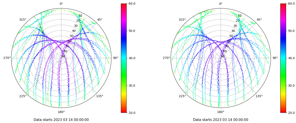
Skyplot for station VIGO. Signal to Noise S1C Data file VIGO00ESP_R_2023073.xtr Skyplot for station VIGO. Signal to Noise S2C Data file VIGO00ESP_R_2023073.xtr
