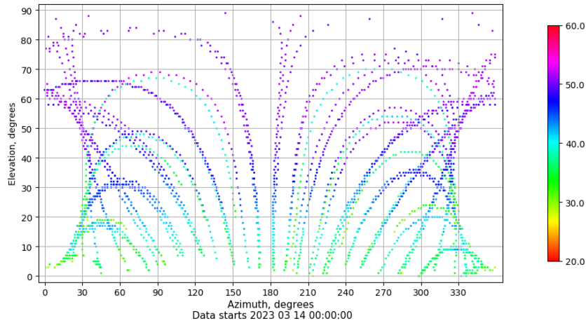
Azimuth-elevation plot for station VIGO. Signal to Noise S1C Data file VIGO00ESP_R_2023073.xtr
