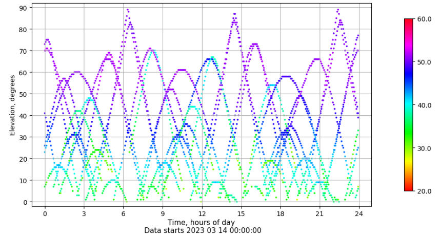
Time-elevation plot for station VIGO. Signal to Noise S1C Data file VIGO00ESP_R_2023073.xtr
