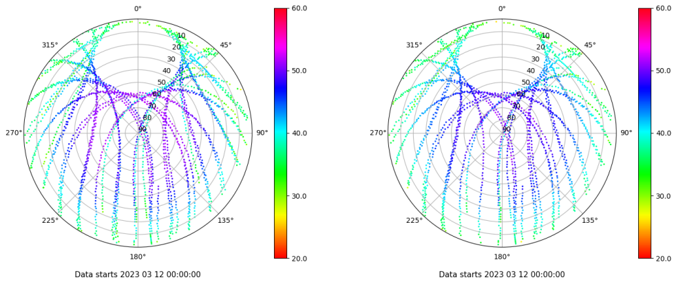
Skyplot for station VIGO. Signal to Noise S1C Data file VIGO00ESP_R_2023071.xtr Skyplot for station VIGO. Signal to Noise S2C Data file VIGO00ESP_R_2023071.xtr
