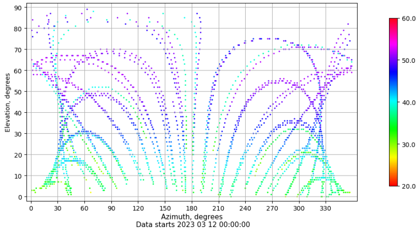
Azimuth-elevation plot for station VIGO. Signal to Noise S1C Data file VIGO00ESP_R_2023071.xtr
