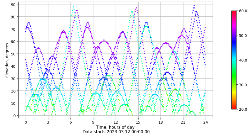
Time-elevation plot for station VIGO. Signal to Noise S1C Data file VIGO00ESP_R_2023071.xtr
