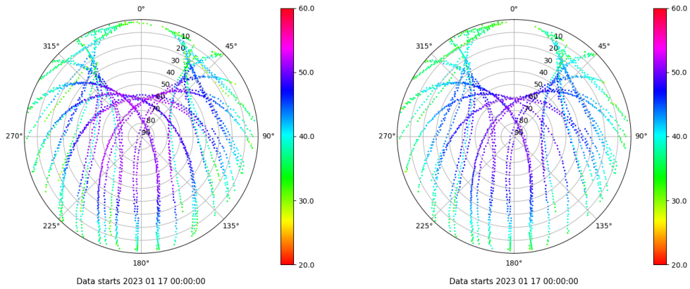
Skyplot for station VIGO. Signal to Noise S1C Data file VIGO00ESP_R_2023017.xtr Skyplot for station VIGO. Signal to Noise S2C Data file VIGO00ESP_R_2023017.xtr
