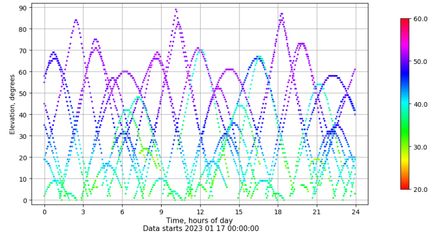
Time-elevation plot for station VIGO. Signal to Noise S1C Data file VIGO00ESP_R_2023017.xtr
