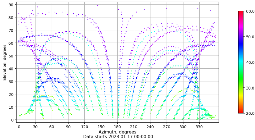
Azimuth-elevation plot for station VIGO. Signal to Noise S1C Data file VIGO00ESP_R_2023017.xtr
