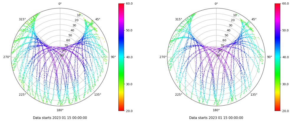
Skyplot for station VIGO. Signal to Noise S1C Data file VIGO00ESP_R_2023015.xtr Skyplot for station VIGO. Signal to Noise S2X Data file VIGO00ESP_R_2023015.xtr
