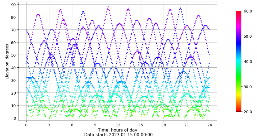
Time-elevation plot for station VIGO. Signal to Noise S1C Data file VIGO00ESP_R_2023015.xtr
