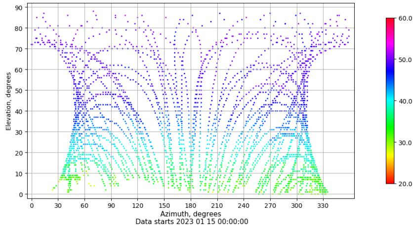
Azimuth-elevation plot for station VIGO. Signal to Noise S1C Data file VIGO00ESP_R_2023015.xtr
