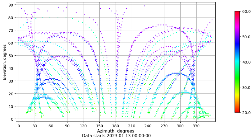
Azimuth-elevation plot for station VIGO. Signal to Noise S1C Data file VIGO00ESP_R_2023013.xtr
