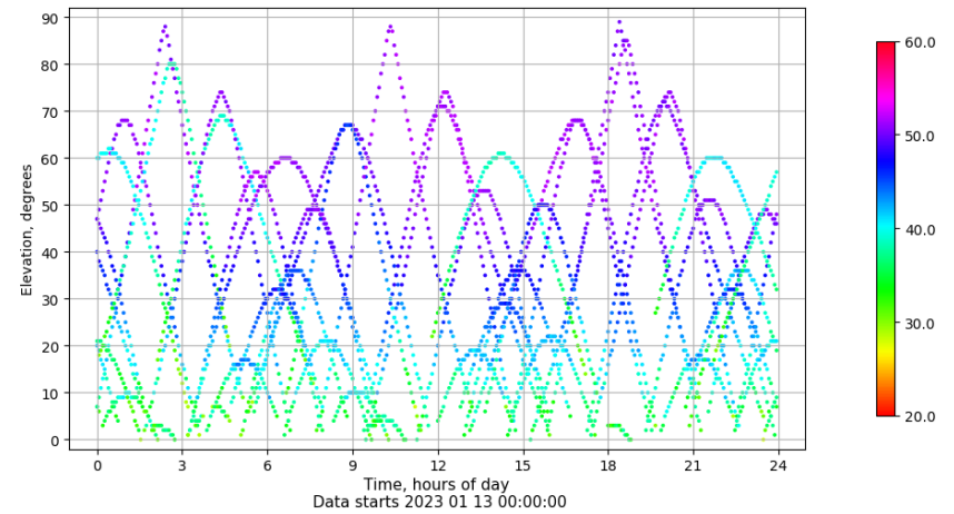
Time-elevation plot for station VIGO. Signal to Noise S1C Data file VIGO00ESP_R_2023013.xtr
