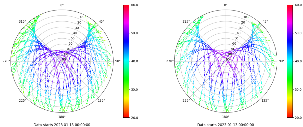
Skyplot for station VIGO. Signal to Noise S1C Data file VIGO00ESP_R_2023013.xtr Skyplot for station VIGO. Signal to Noise S2X Data file VIGO00ESP_R_2023013.xtr
