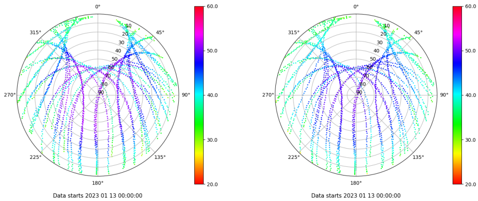
Skyplot for station VIGO. Signal to Noise S1C Data file VIGO00ESP_R_2023013.xtr Skyplot for station VIGO. Signal to Noise S2C Data file VIGO00ESP_R_2023013.xtr
