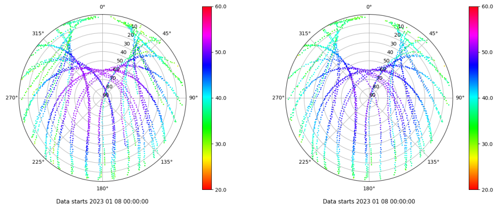
Skyplot for station VIGO. Signal to Noise S1C Data file VIGO00ESP_R_2023008.xtr Skyplot for station VIGO. Signal to Noise S2C Data file VIGO00ESP_R_2023008.xtr
