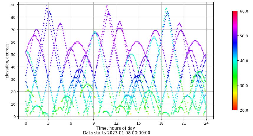
Time-elevation plot for station VIGO. Signal to Noise S1C Data file VIGO00ESP_R_2023008.xtr
