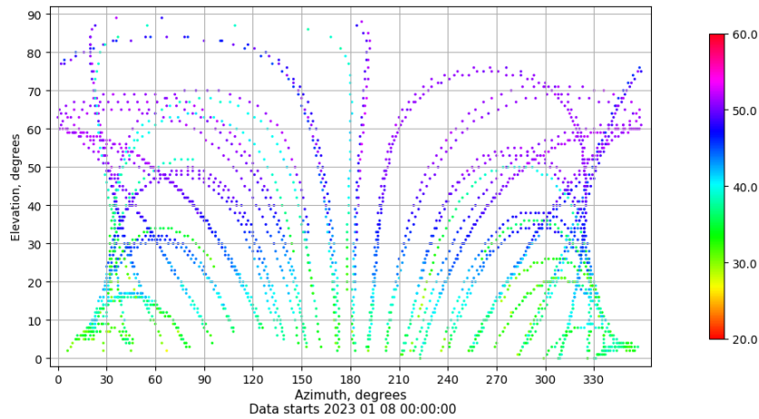
Azimuth-elevation plot for station VIGO. Signal to Noise S1C Data file VIGO00ESP_R_2023008.xtr
