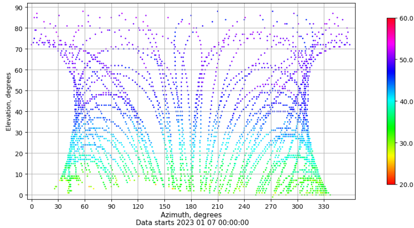
Azimuth-elevation plot for station VIGO. Signal to Noise S1C Data file VIGO00ESP_R_2023007.xtr
