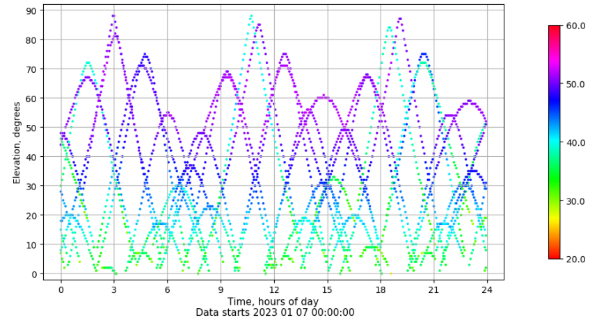
Time-elevation plot for station VIGO. Signal to Noise S1C Data file VIGO00ESP_R_2023007.xtr
