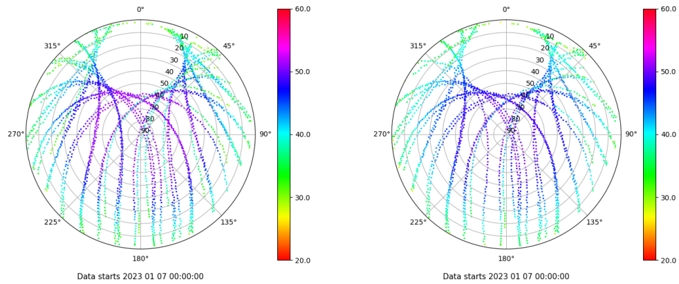
Skyplot for station VIGO. Signal to Noise S1C Data file VIGO00ESP_R_2023007.xtr Skyplot for station VIGO. Signal to Noise S2C Data file VIGO00ESP_R_2023007.xtr
