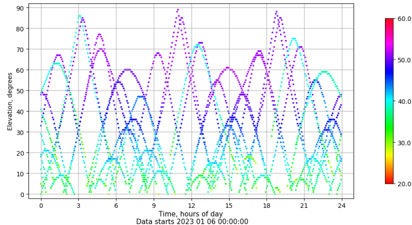
Time-elevation plot for station VIGO. Signal to Noise S1C Data file VIGO00ESP_R_2023006.xtr
