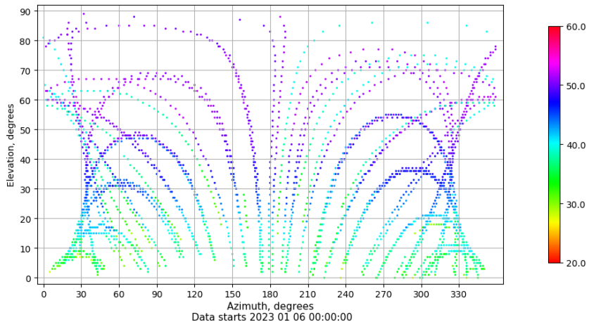
Azimuth-elevation plot for station VIGO. Signal to Noise S1C Data file VIGO00ESP_R_2023006.xtr
