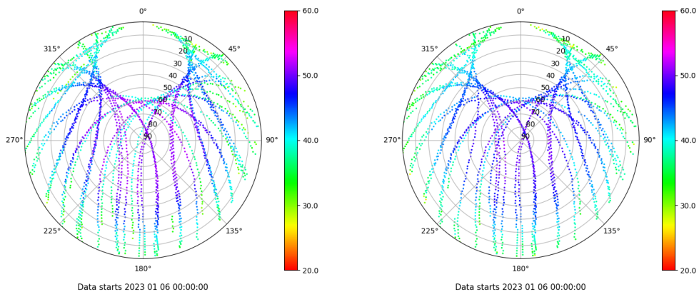
Skyplot for station VIGO. Signal to Noise S1C Data file VIGO00ESP_R_2023006.xtr Skyplot for station VIGO. Signal to Noise S2C Data file VIGO00ESP_R_2023006.xtr
