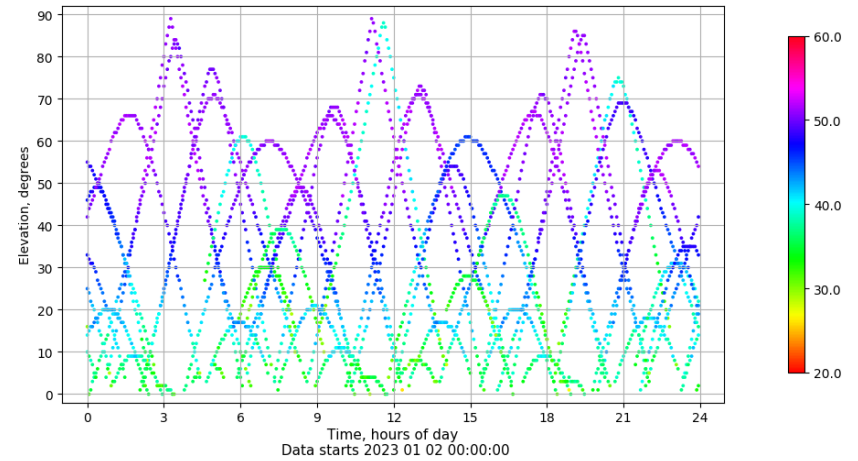
Time-elevation plot for station VIGO. Signal to Noise S1C Data file VIGO00ESP_R_2023002.xtr
