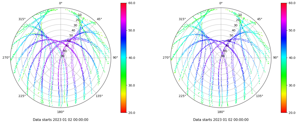
Skyplot for station VIGO. Signal to Noise S1C Data file VIGO00ESP_R_2023002.xtr Skyplot for station VIGO. Signal to Noise S2C Data file VIGO00ESP_R_2023002.xtr
