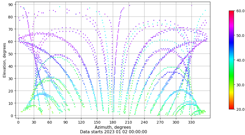
Azimuth-elevation plot for station VIGO. Signal to Noise S1C Data file VIGO00ESP_R_2023002.xtr
