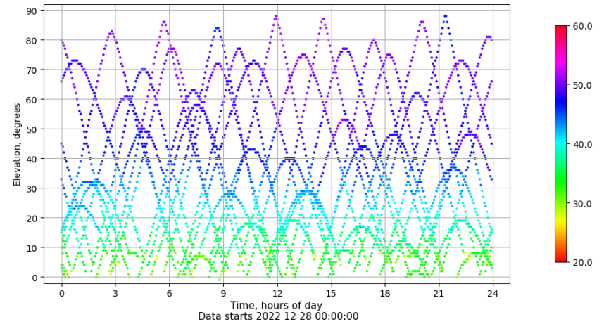
Time-elevation plot for station VIGO. Signal to Noise S1C Data file VIGO00ESP_R_2022362.xtr
