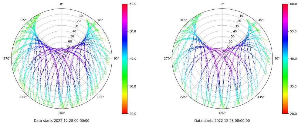
Skyplot for station VIGO. Signal to Noise S1C Data file VIGO00ESP_R_2022362.xtr Skyplot for station VIGO. Signal to Noise S2X Data file VIGO00ESP_R_2022362.xtr
