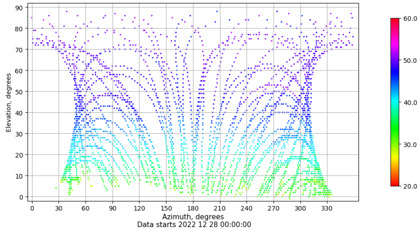
Azimuth-elevation plot for station VIGO. Signal to Noise S1C Data file VIGO00ESP_R_2022362.xtr
