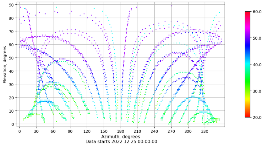
Azimuth-elevation plot for station VIGO. Signal to Noise S1C Data file VIGO00ESP_R_2022359.xtr
