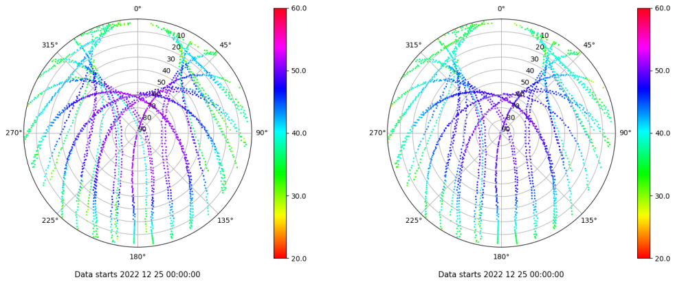
Skyplot for station VIGO. Signal to Noise S1C Data file VIGO00ESP_R_2022359.xtr Skyplot for station VIGO. Signal to Noise S2C Data file VIGO00ESP_R_2022359.xtr
