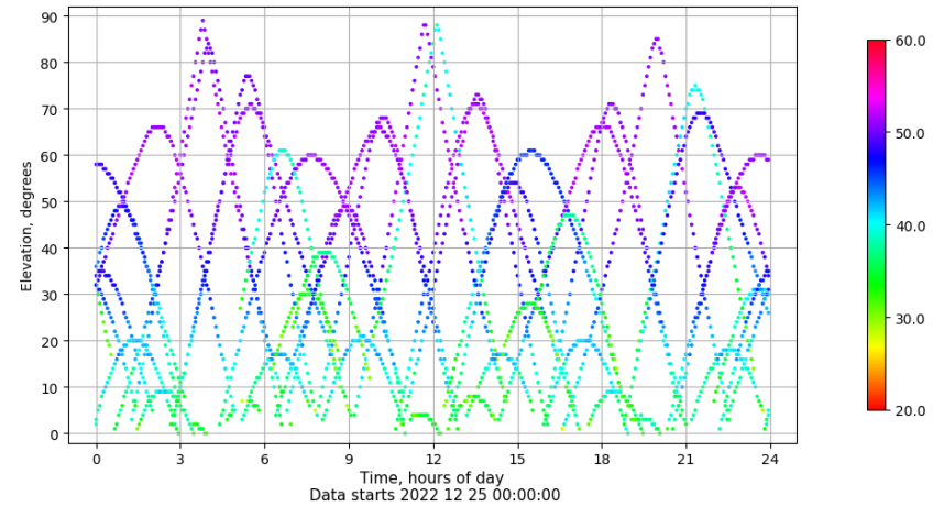
Time-elevation plot for station VIGO. Signal to Noise S1C Data file VIGO00ESP_R_2022359.xtr
