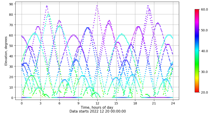
Time-elevation plot for station VIGO. Signal to Noise S1C Data file VIGO00ESP_R_2022354.xtr
