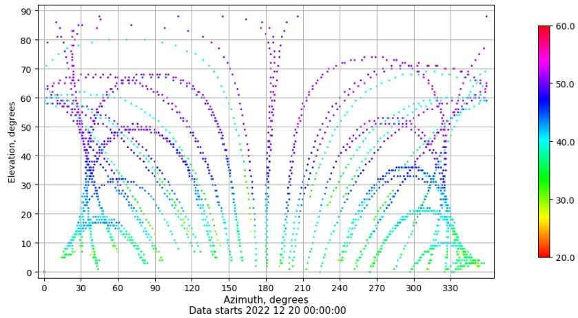
Azimuth-elevation plot for station VIGO. Signal to Noise S1C Data file VIGO00ESP_R_2022354.xtr
