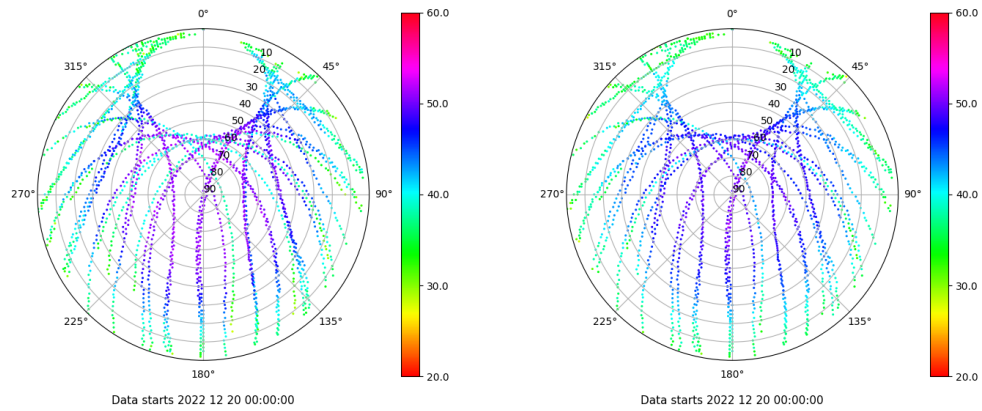
Skyplot for station VIGO. Signal to Noise S1C Data file VIGO00ESP_R_2022354.xtr Skyplot for station VIGO. Signal to Noise S2C Data file VIGO00ESP_R_2022354.xtr
