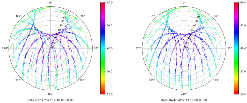
Skyplot for station VIGO. Signal to Noise S1C Data file VIGO00ESP_R_2022352.xtr Skyplot for station VIGO. Signal to Noise S2C Data file VIGO00ESP_R_2022352.xtr
