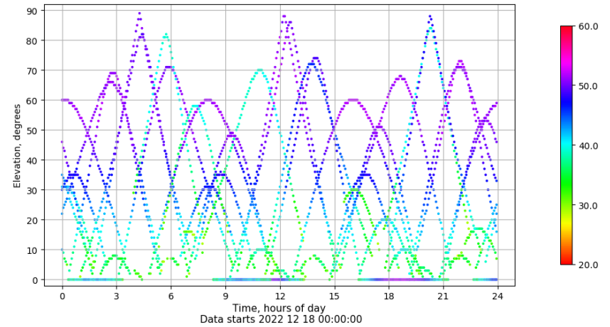
Time-elevation plot for station VIGO. Signal to Noise S1C Data file VIGO00ESP_R_2022352.xtr
