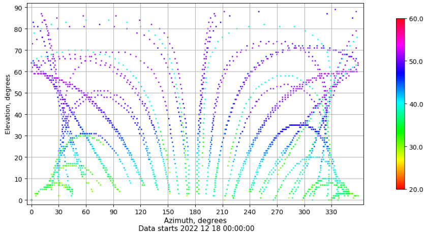
Azimuth-elevation plot for station VIGO. Signal to Noise S1C Data file VIGO00ESP_R_2022352.xtr
