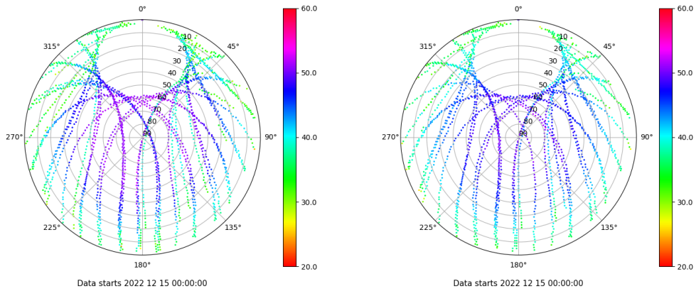
Skyplot for station VIGO. Signal to Noise S1C Data file VIGO00ESP_R_2022349.xtr Skyplot for station VIGO. Signal to Noise S2C Data file VIGO00ESP_R_2022349.xtr
