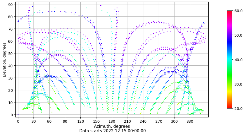
Azimuth-elevation plot for station VIGO. Signal to Noise S1C Data file VIGO00ESP_R_2022349.xtr
