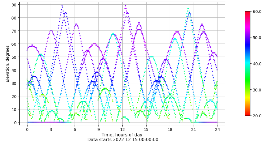
Time-elevation plot for station VIGO. Signal to Noise S1C Data file VIGO00ESP_R_2022349.xtr
