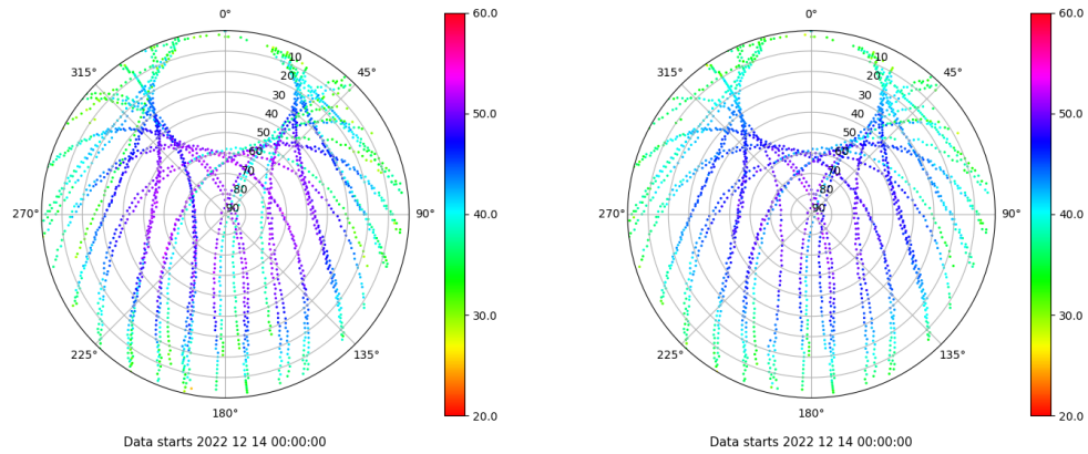
Skyplot for station VIGO. Signal to Noise S1C Data file VIGO00ESP_R_2022348.xtr Skyplot for station VIGO. Signal to Noise S2C Data file VIGO00ESP_R_2022348.xtr
