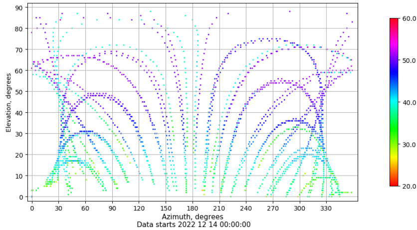
Azimuth-elevation plot for station VIGO. Signal to Noise S1C Data file VIGO00ESP_R_2022348.xtr
