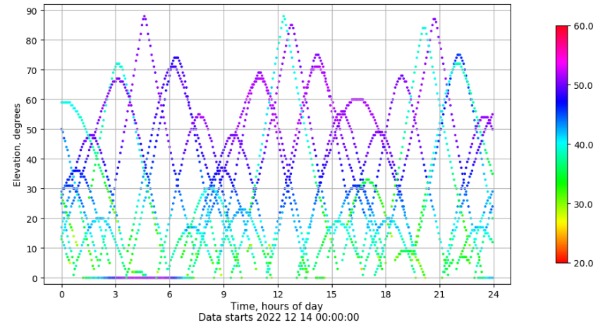
Time-elevation plot for station VIGO. Signal to Noise S1C Data file VIGO00ESP_R_2022348.xtr
