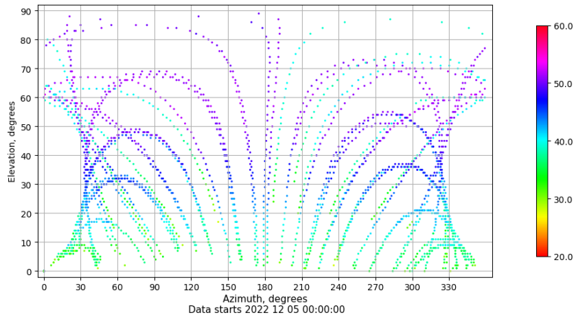
Azimuth-elevation plot for station VIGO. Signal to Noise S1C Data file VIGO00ESP_R_2022339.xtr
