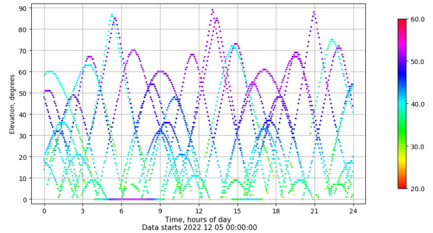
Time-elevation plot for station VIGO. Signal to Noise S1C Data file VIGO00ESP_R_2022339.xtr
