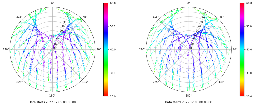
Skyplot for station VIGO. Signal to Noise S1C Data file VIGO00ESP_R_2022339.xtr Skyplot for station VIGO. Signal to Noise S2C Data file VIGO00ESP_R_2022339.xtr
