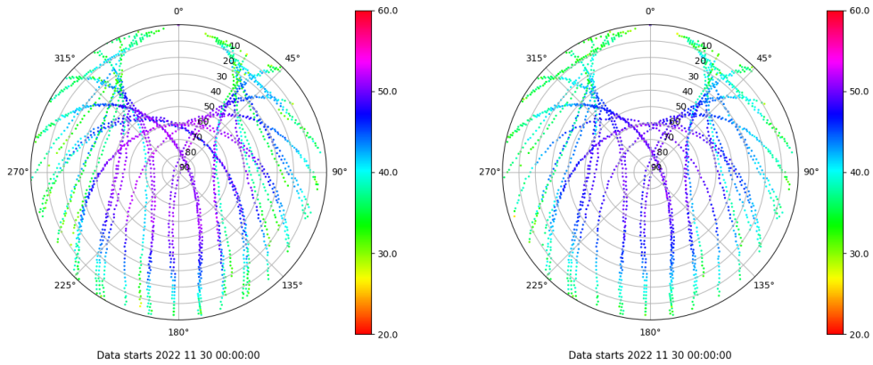
Skyplot for station VIGO. Signal to Noise S1C Data file VIGO00ESP_R_2022334.xtr Skyplot for station VIGO. Signal to Noise S2C Data file VIGO00ESP_R_2022334.xtr
