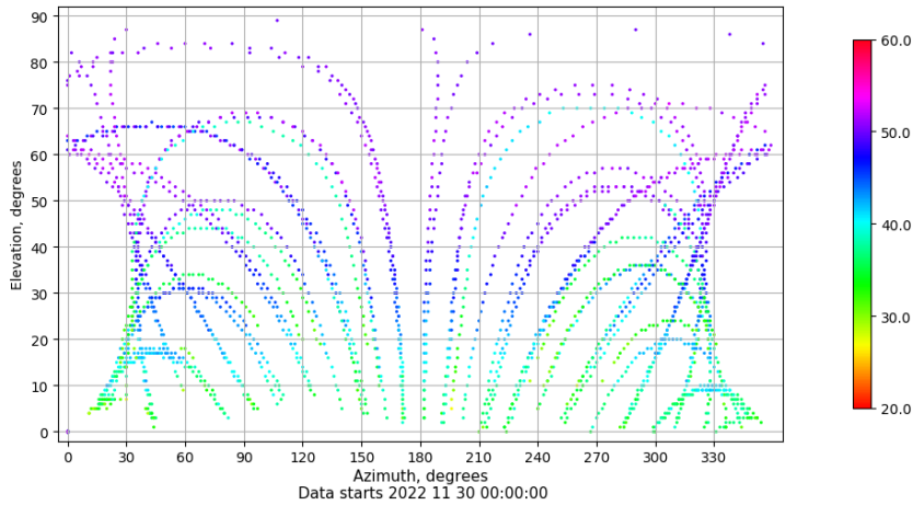
Azimuth-elevation plot for station VIGO. Signal to Noise S1C Data file VIGO00ESP_R_2022334.xtr
