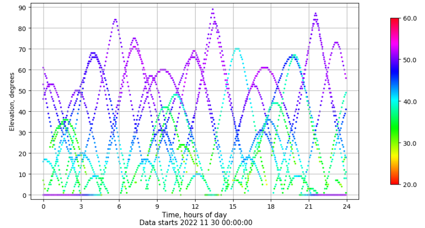
Time-elevation plot for station VIGO. Signal to Noise S1C Data file VIGO00ESP_R_2022334.xtr
