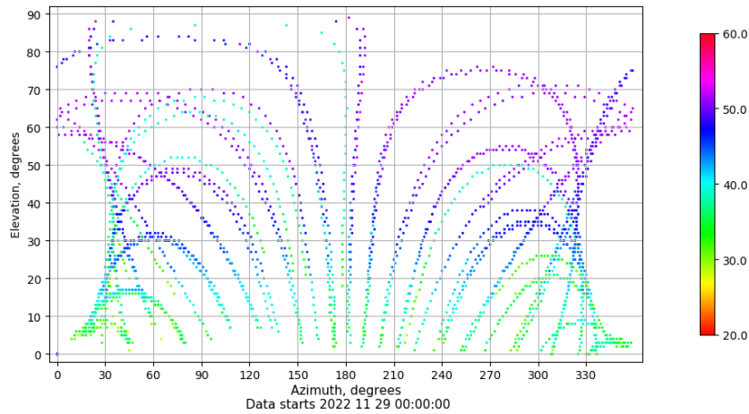
Azimuth-elevation plot for station VIGO. Signal to Noise S1C Data file VIGO00ESP_R_2022333.xtr
