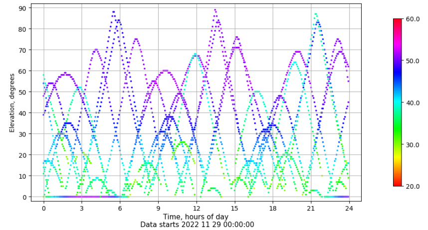
Time-elevation plot for station VIGO. Signal to Noise S1C Data file VIGO00ESP_R_2022333.xtr
