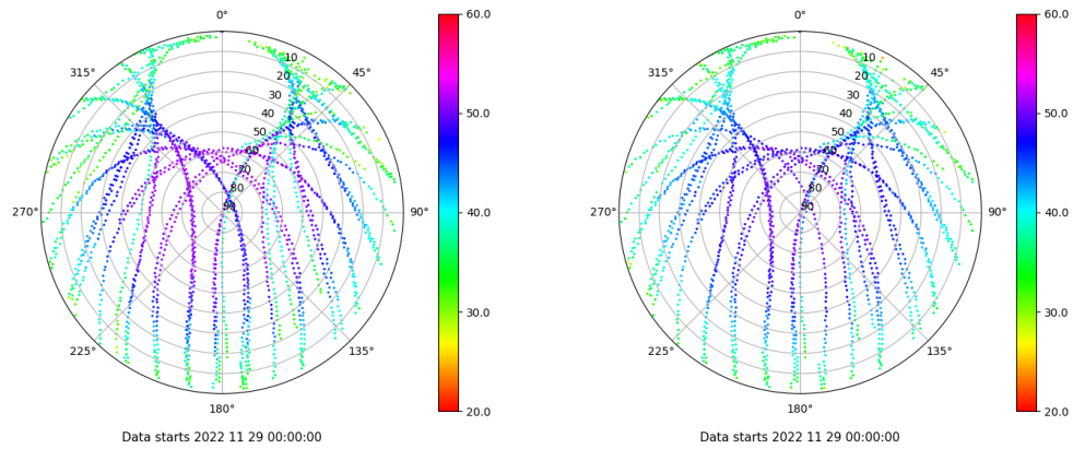
Skyplot for station VIGO. Signal to Noise S1C Data file VIGO00ESP_R_2022333.xtr Skyplot for station VIGO. Signal to Noise S2C Data file VIGO00ESP_R_2022333.xtr
