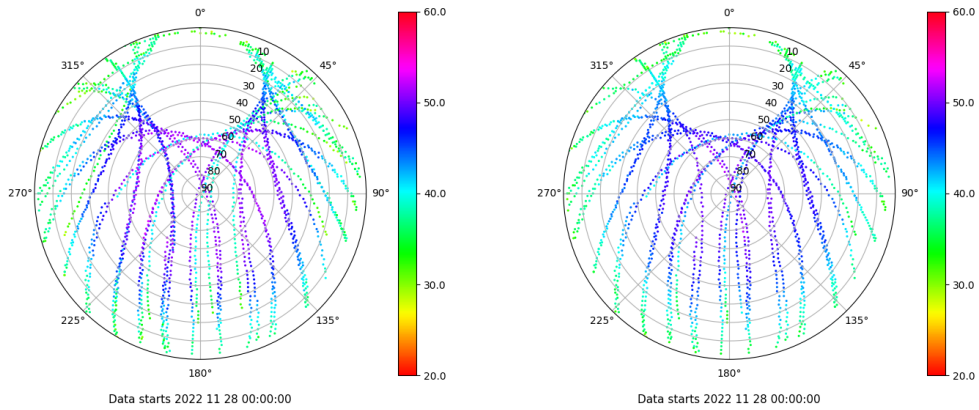
Skyplot for station VIGO. Signal to Noise S1C Data file VIGO00ESP_R_2022332.xtr Skyplot for station VIGO. Signal to Noise S2C Data file VIGO00ESP_R_2022332.xtr
