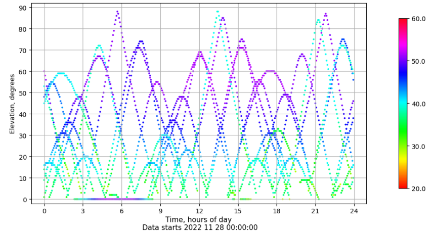
Time-elevation plot for station VIGO. Signal to Noise S1C Data file VIGO00ESP_R_2022332.xtr
