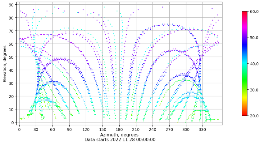
Azimuth-elevation plot for station VIGO. Signal to Noise S1C Data file VIGO00ESP_R_2022332.xtr
